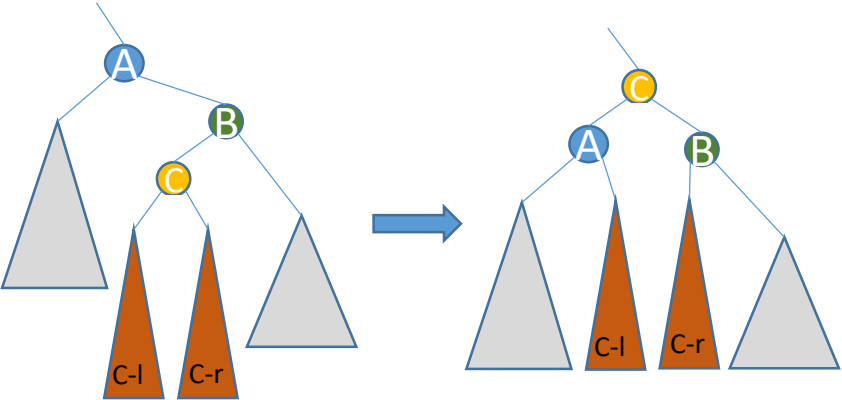
Right-Left Rotation
