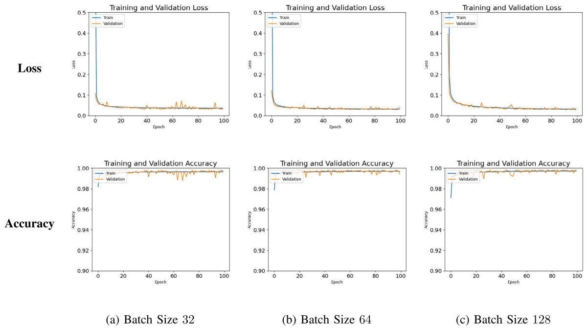
(a) LSTM 16-16-16 model plots for binary classification.
