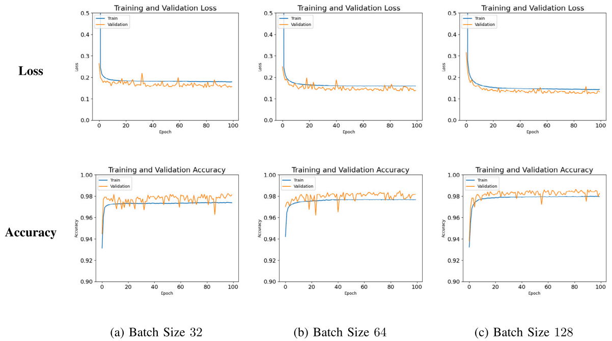
(a) LSTM 256-256-128 model plots for multiclass classification.
