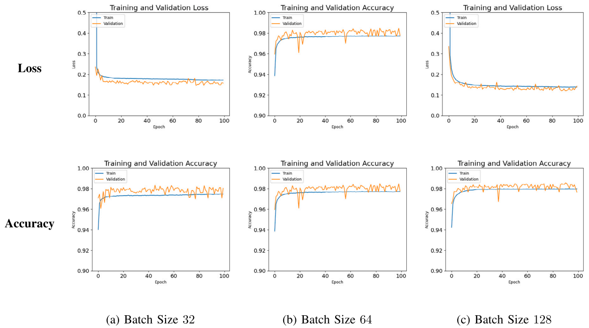
(a) LSTM 128-128-128 model plots for multiclass classification.
